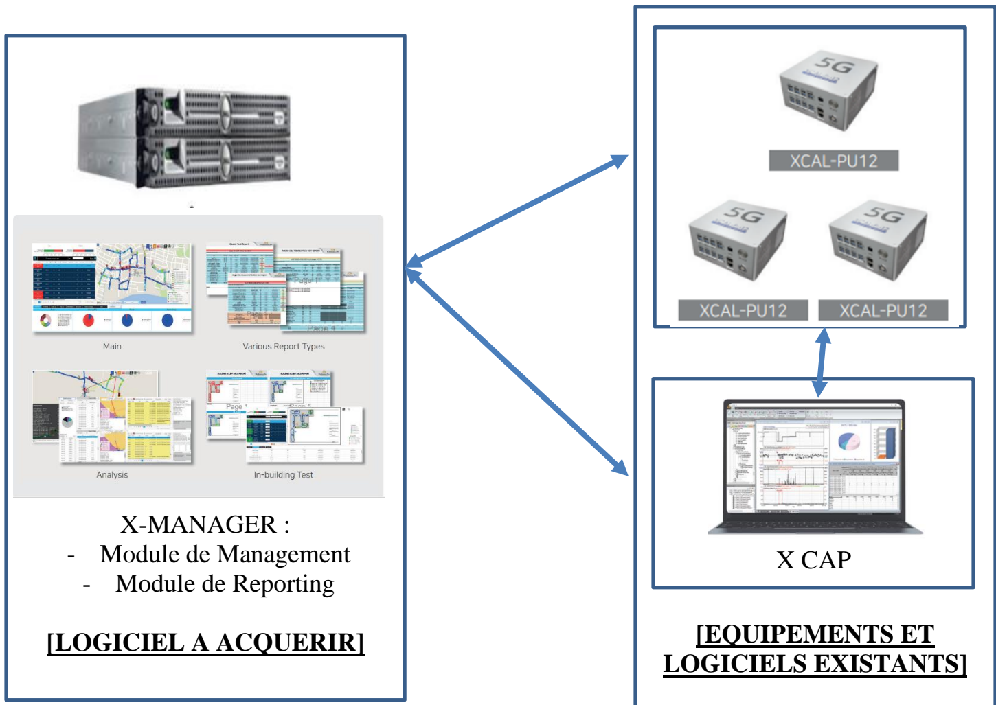
Figure 1: Architecture cible
